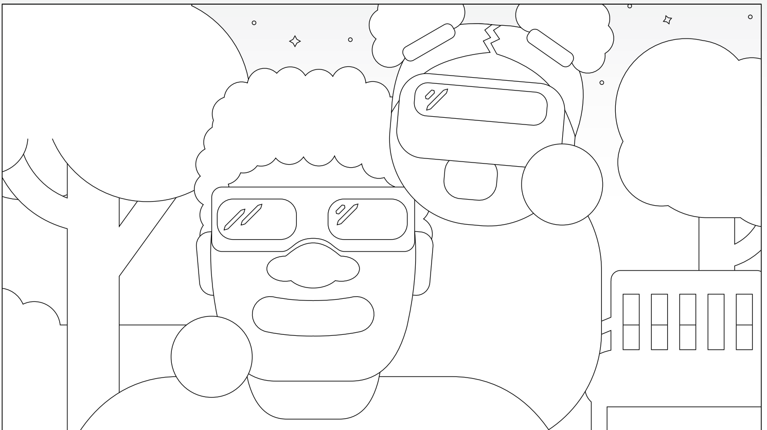
Partial Eclipse
