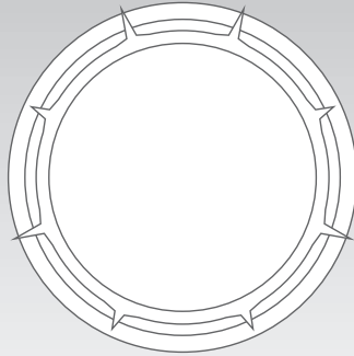
Annular Eclipse
