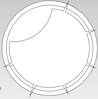
Partial Eclipse
