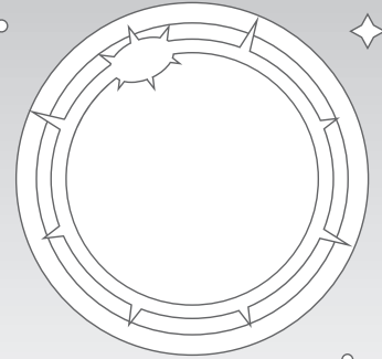
Total Eclipse
